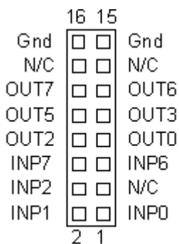
16 pin Header - Top View
