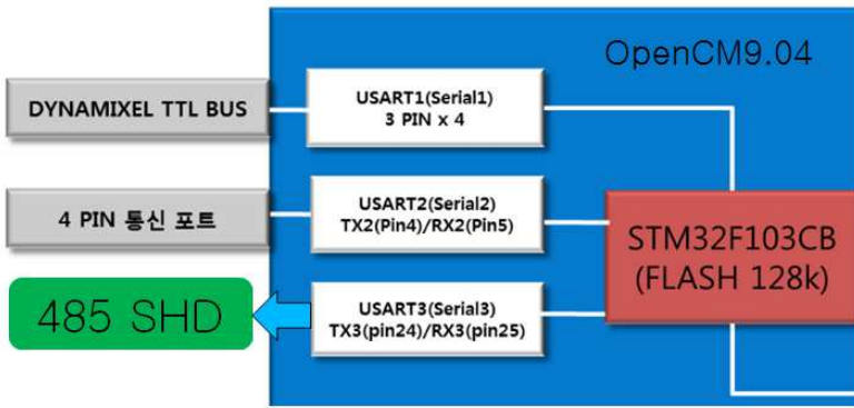
[ OpenCM9.04 & OpenCM 485 EXP Bus Connections ]
