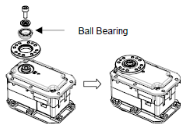
HN05-I1(Bearing Set RX-64H)
